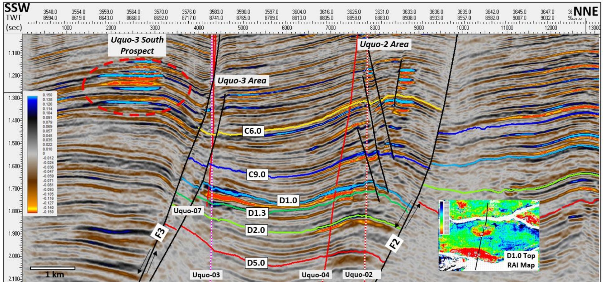
Figure 3-5 SW-NNE seismic line through Uquo-3 and Uquo-2 areas (Source: Savannah, 2021)
