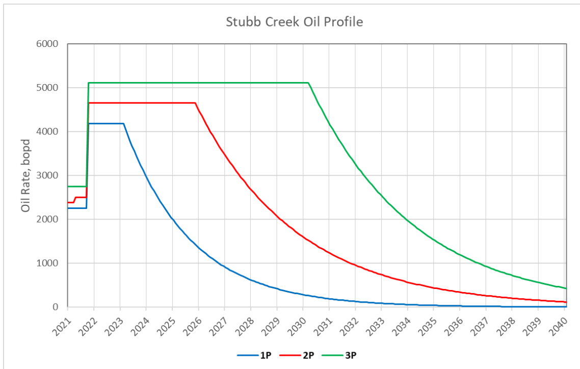
Figure 4-4 Stubb Creek production forecast profiles
