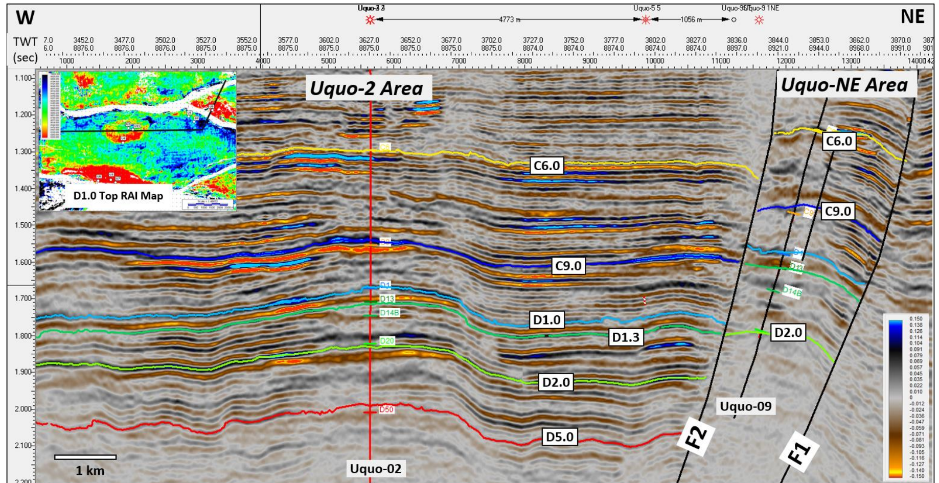
Figure 3-7 E-W Seismic crossline for Uquo-2 and Uquo-NE area showing tops of target units. See inset map for location (Source: Savannah, 2021)
