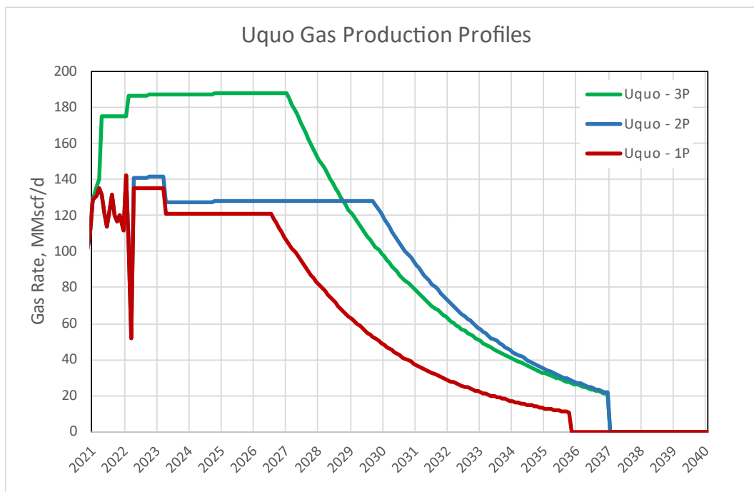
Figure 4-2 Uquo field production forecast profiles (Reserves cases)
